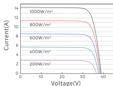
Current-Voltage Curve JAM54D40-450/LB/1500V
