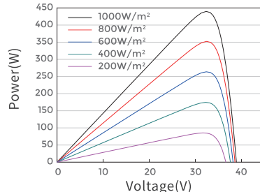
Power-Voltage Curve JAM54D40-450/LB/1500V
