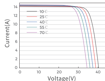
Current-Voltage Curve JAM54D40-450/LB/1500V
